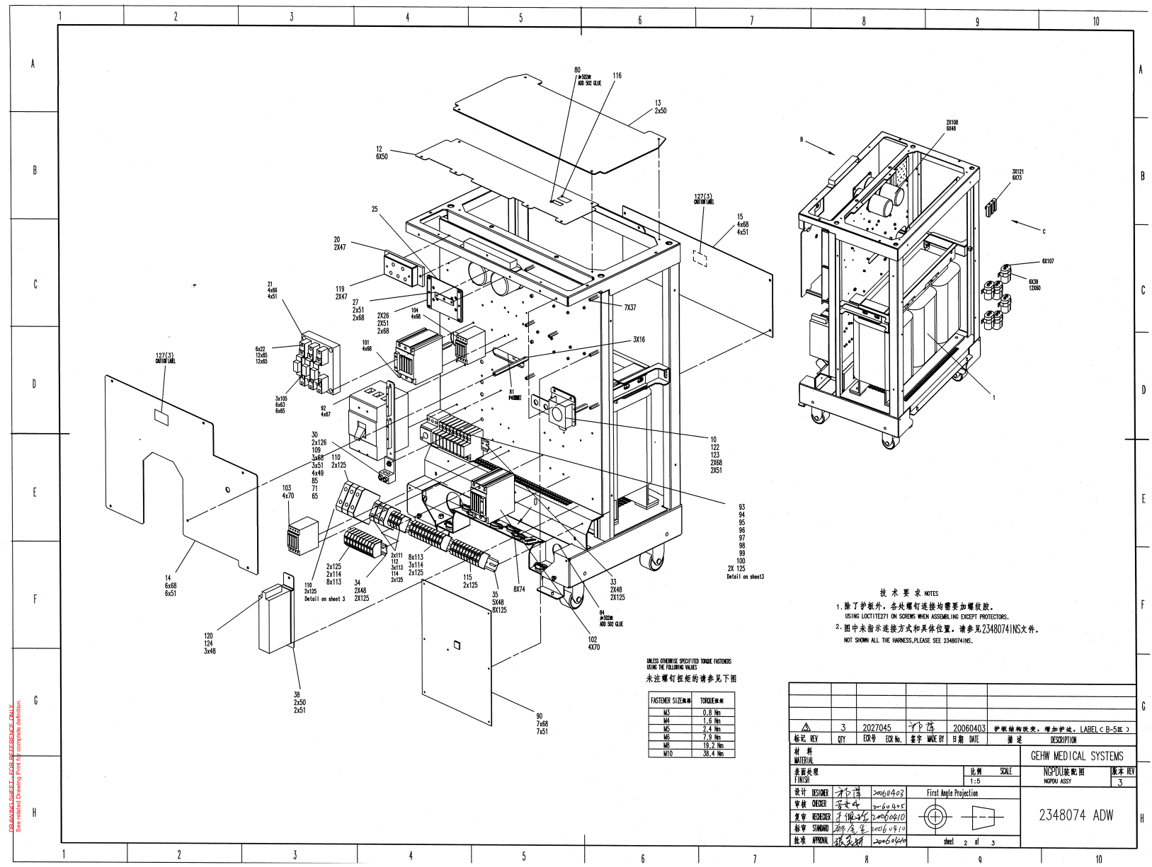
Figure 3-2 NGPDU Assembly 1 (2348074, sheet 2, rev 3)
