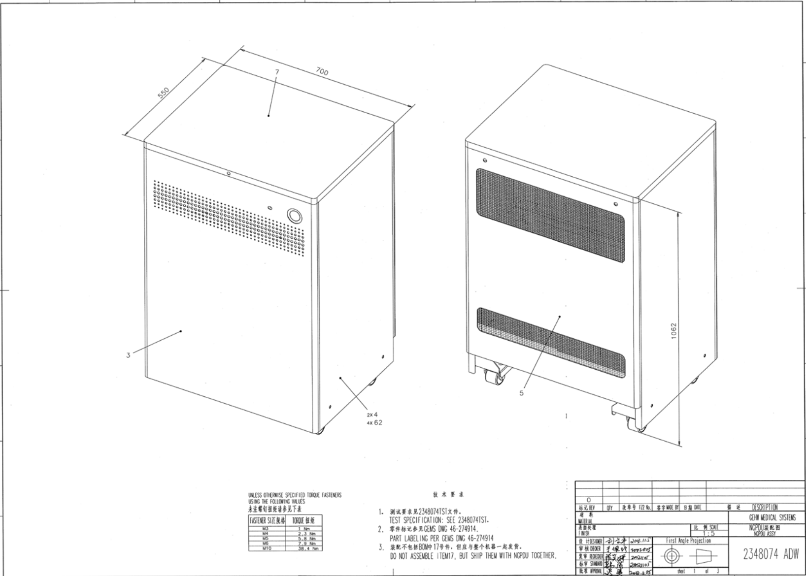
Figure 3-1 NGPDU Assembly 1 (2348074, sheet 1, rev 0)
